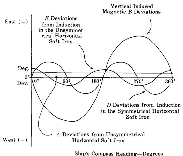
Figure 307b – Induced magnetic deviation effects
