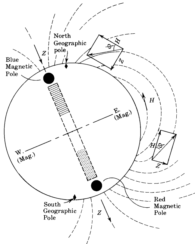
Figure 205 – Terrestrial magnetism
