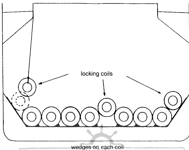
Figure 9 – Inserting of locking coils
