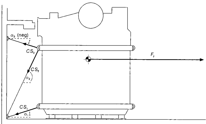
Figure 17 – Balance of transverse forces
