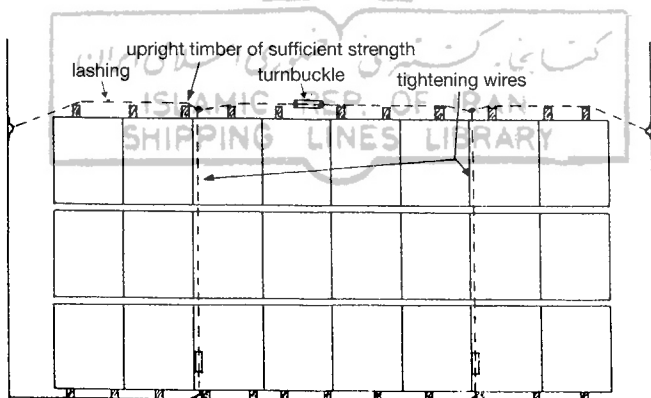
Figure 13 – Securing of end row in top tier against fore-and-aft shifting (view from top)
