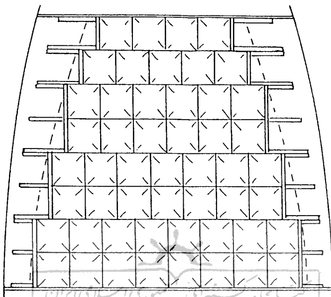
Figure 15 – Stowage and chocking of unit loads in a tapered stowage area (view from top)
