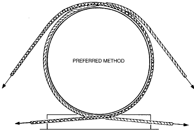
Figure 4 – Securing of portable tanks having no securing points
