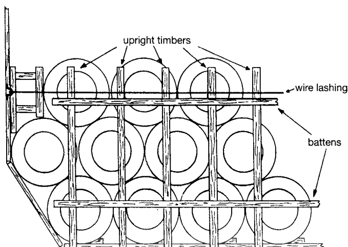
Figure 12 – Securing of end row in top tier against fore-and-aft shifting
