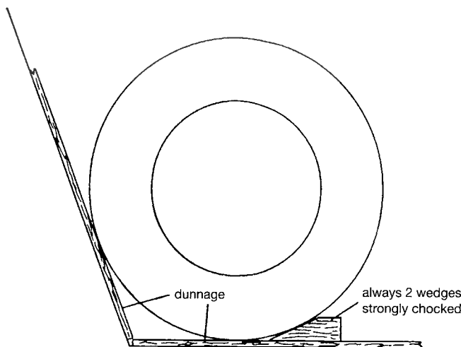
Figure 8 – Principle of dunnaging and wedging coils
