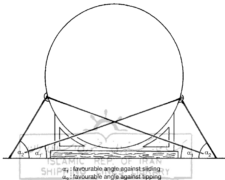
Figure 3 – Securing of portable tanks with favourable lashing angles
