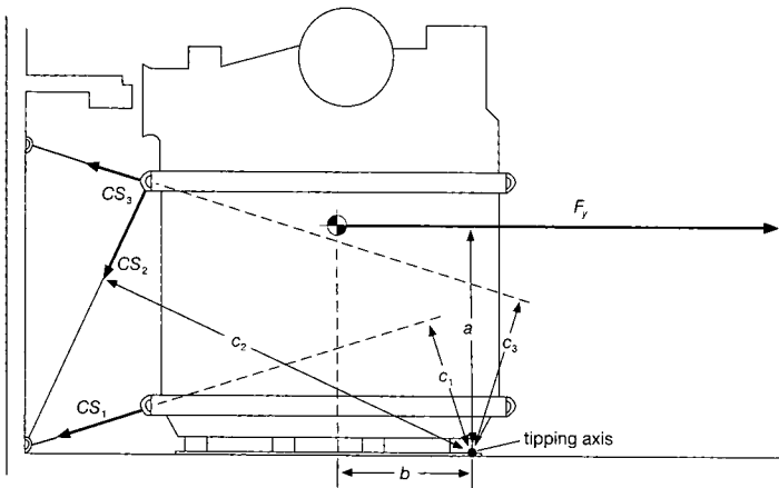
Figure 18 – Balance of transverse moments
