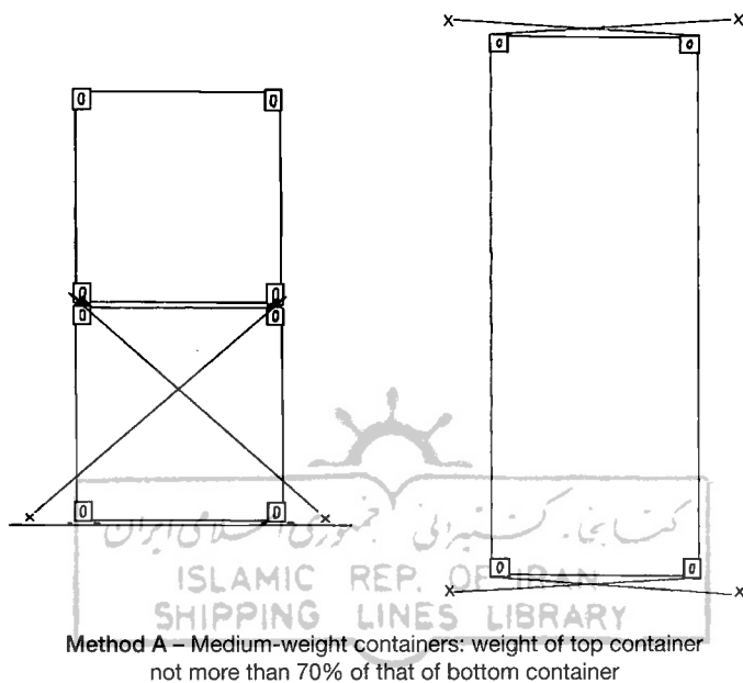
Figure 1 – Recommended methods of non-standardized ... securing of containers
