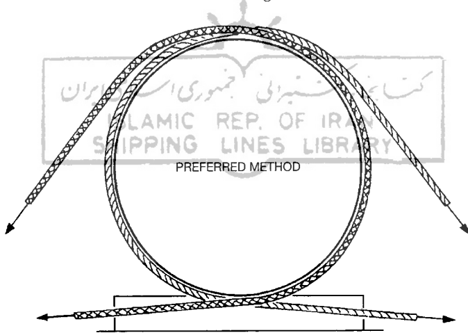
Figure 7 – Principle of securing heavy items having no suitable securing points
