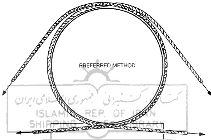
Figure 5 – Securing of receptacles having no securing points
