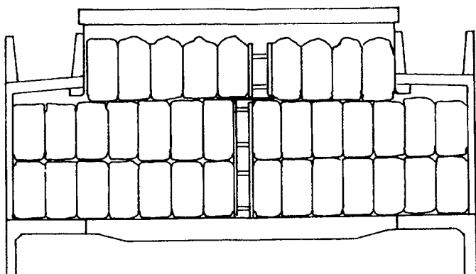
Figure 14 – Stowage of FIBCs with chocked void spaces in the centre of the stowage area
