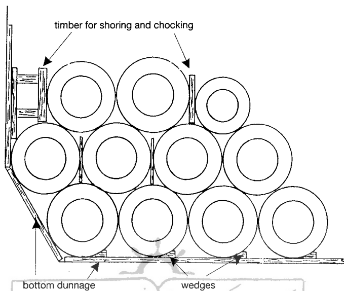
Figure 10 – Shoring and chocking in voids between coils
