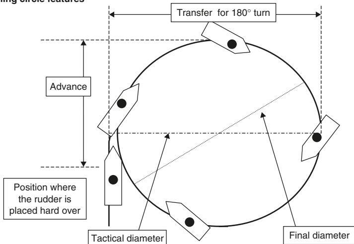
Turning circle features
