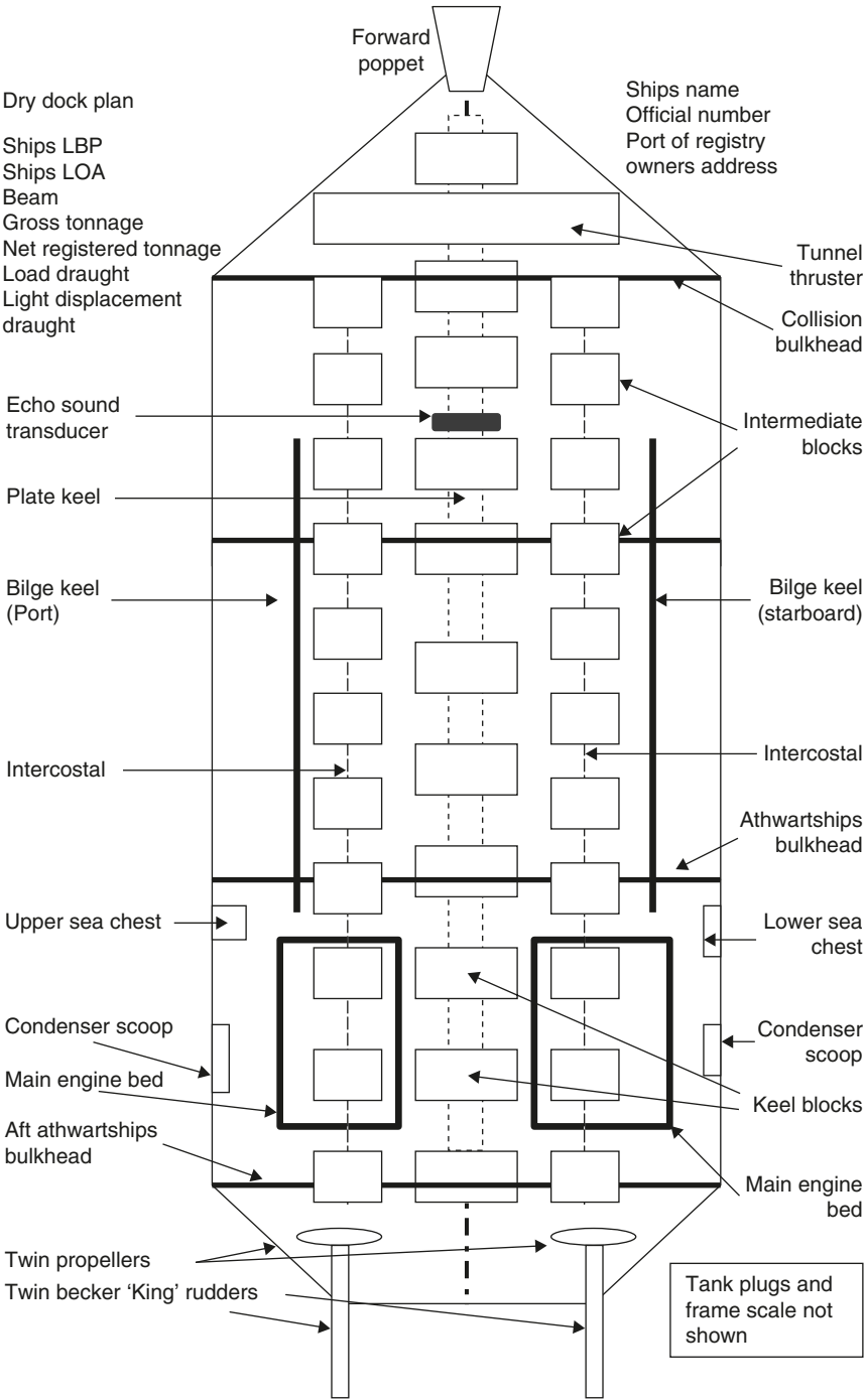
Dry Dock Plan.
