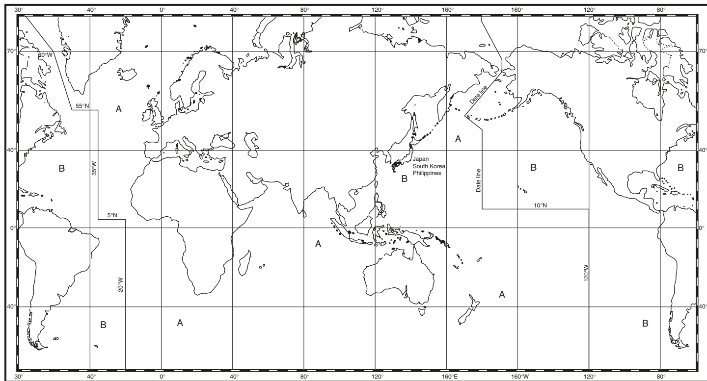
The IALA Maritime Buoyage Systems – Regions A and B. Reproduced with permission from IALA.
