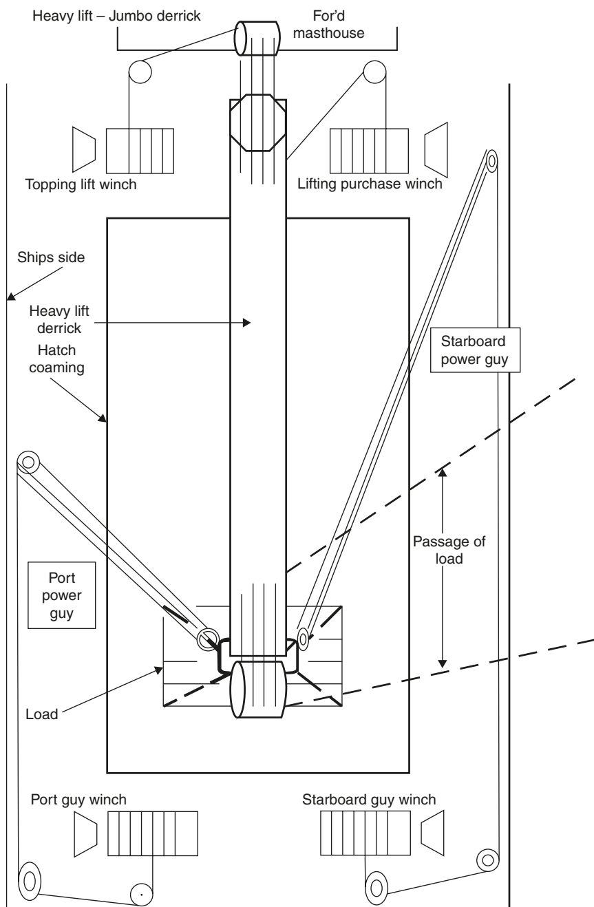
Heavy lift - Jumbo derrick.
