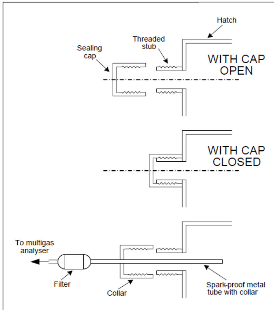
Diagram of gas sampling point
