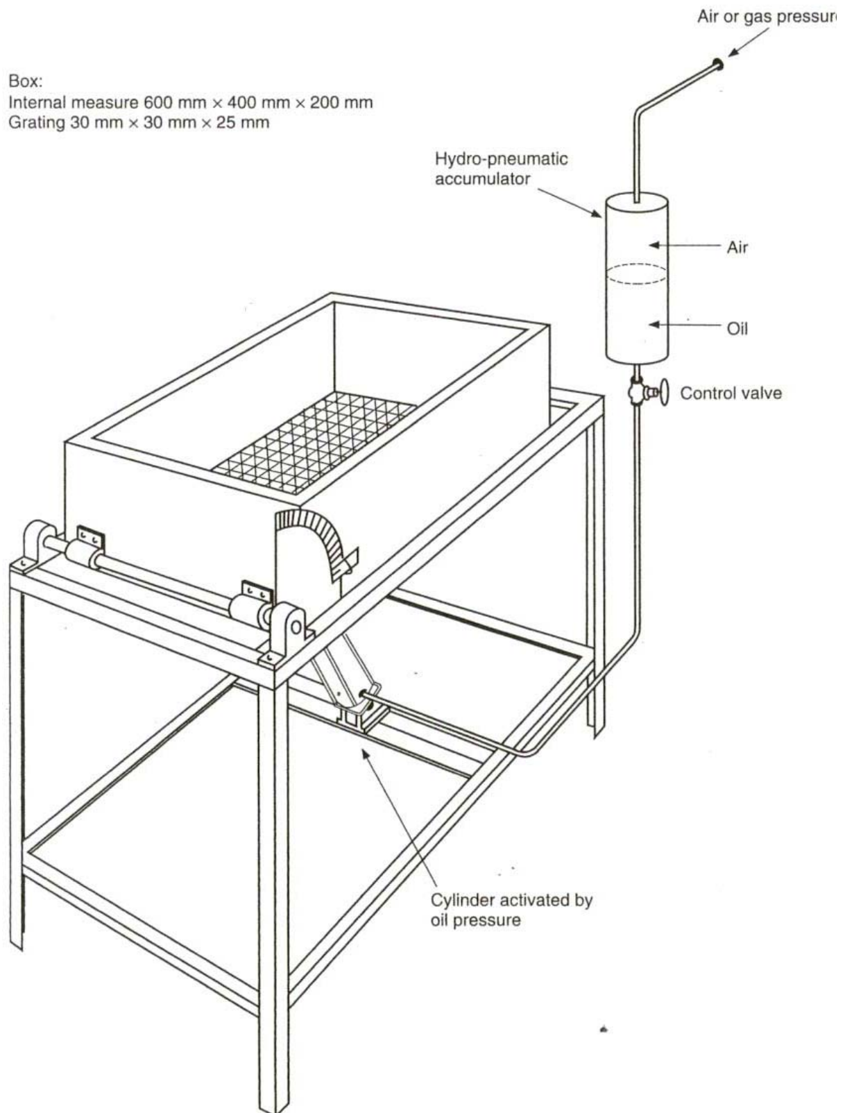
Figure 2.1.4 . Basic sketch of tilting box
