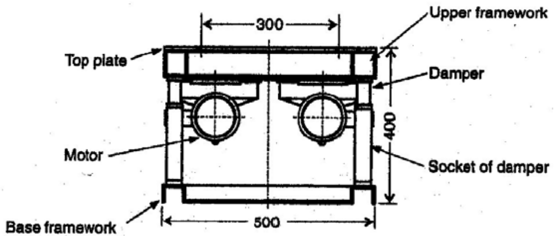
Figure 1.2.2 . Test apparatus FRONT VIEW
