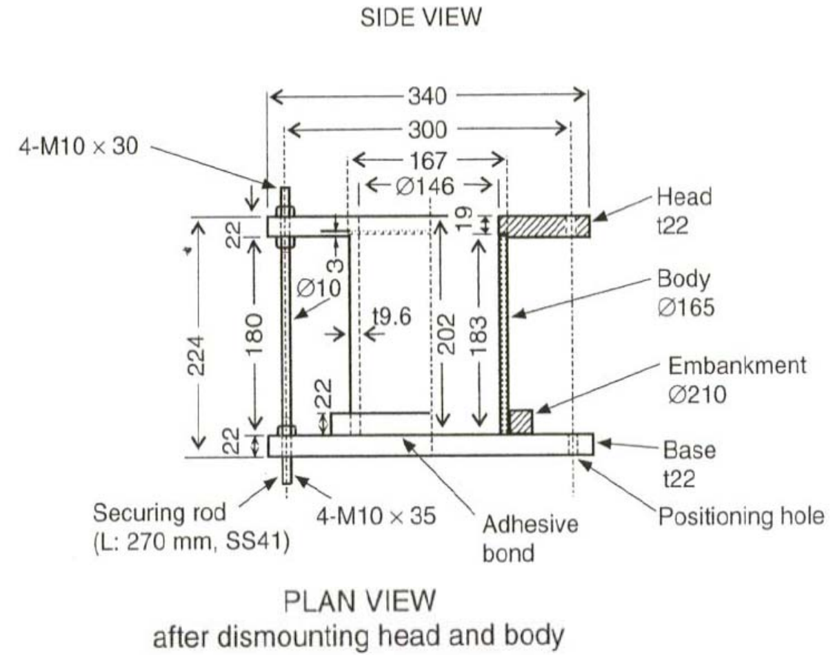
Figure 1.2.2.2 . Vibration table
