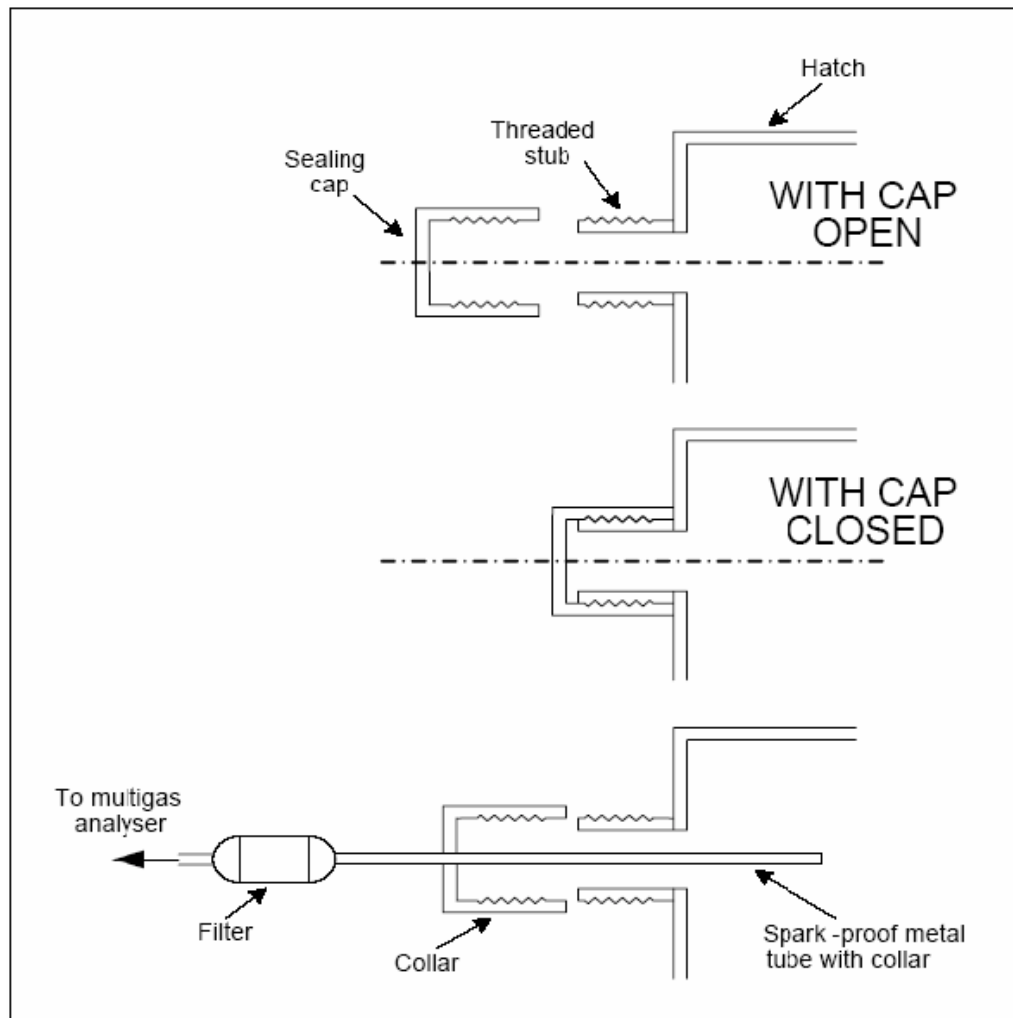
Diagram of gas sampling point
