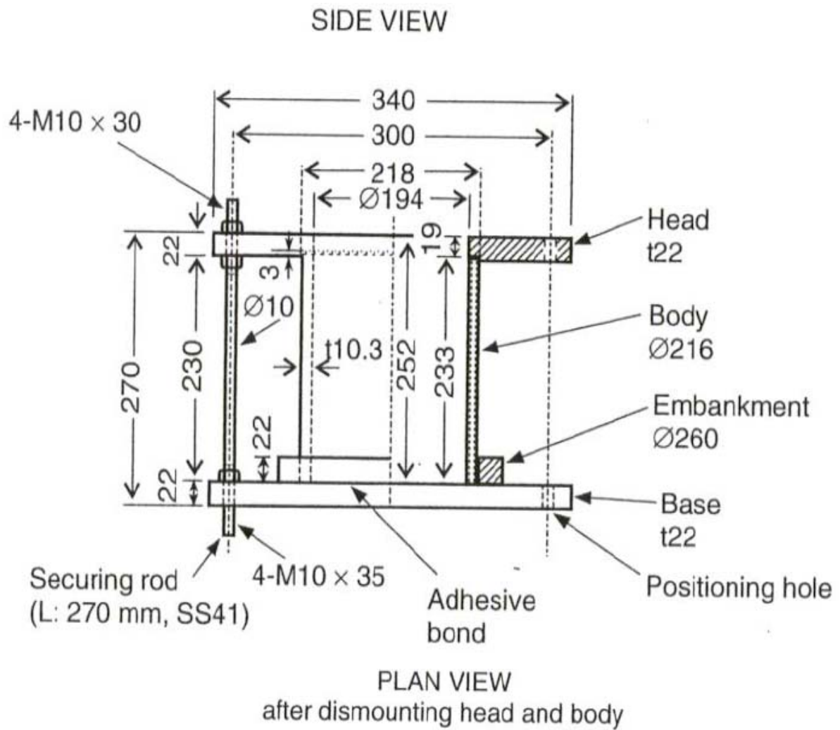
Figure 1.2.2.3-1 . Cylindrical vessel, 150 mm diameter
