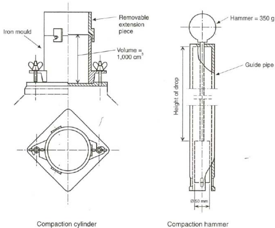
Figure 1.3.2 . Proctor apparatus
